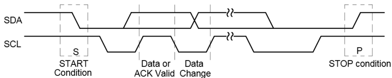
Figure 3-5-2. Data Transmission Sequence
