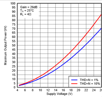
Figure 14. Maximum Output Power (BTL) vs Supply Voltage
