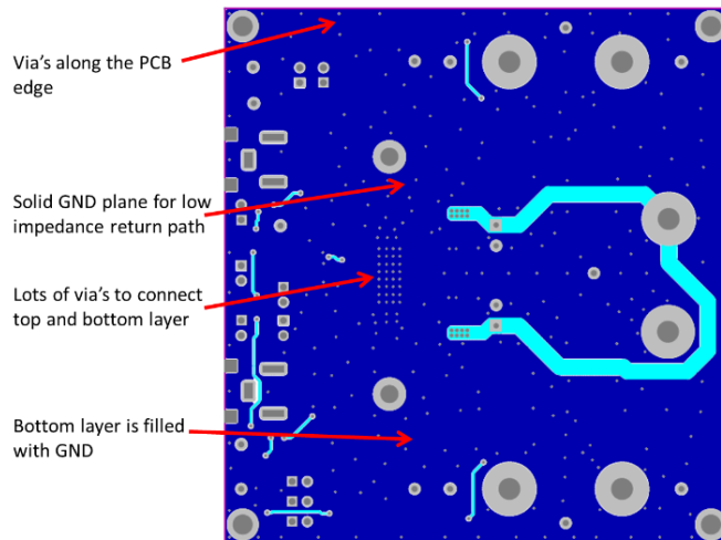
Figure 41. Layout Example Bottom
