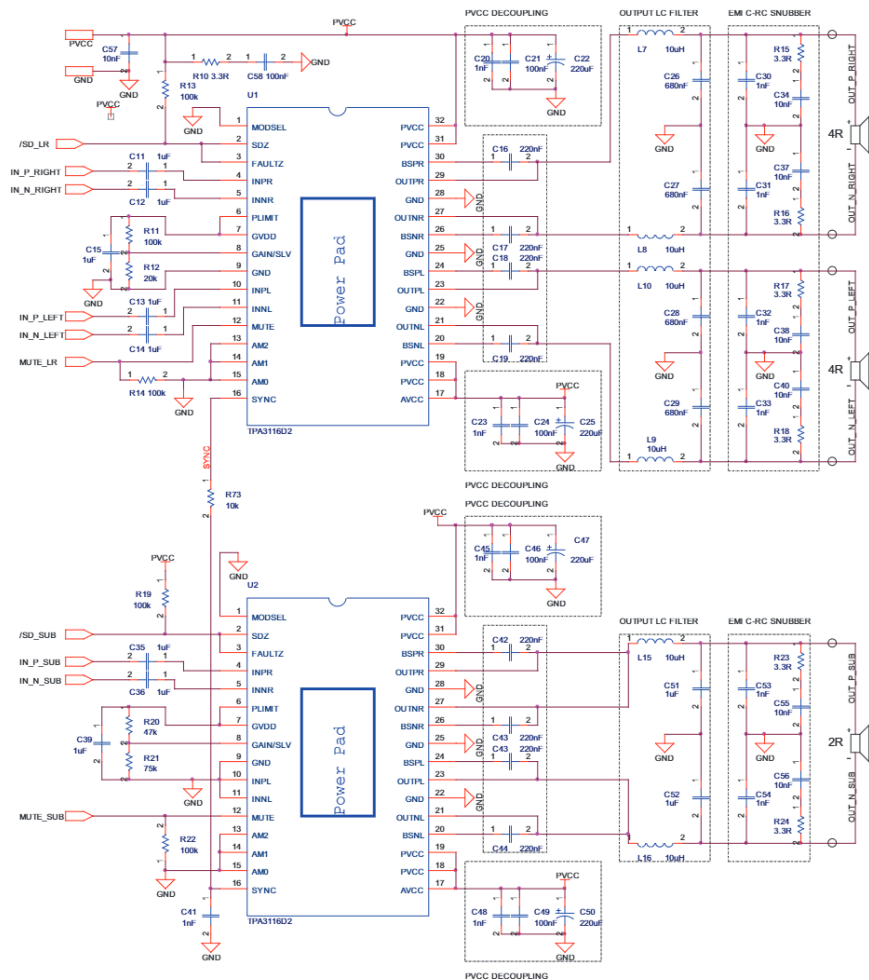
Figure 37. Schematic
