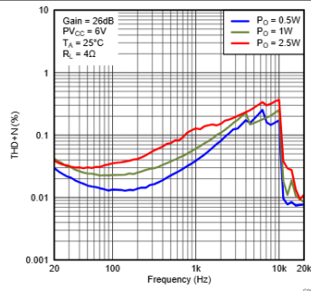
Figure 1. Total Harmonic Distortion + Noise (BTL) vs Frequency
