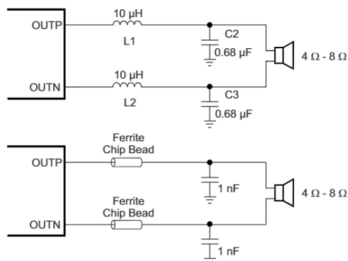
Figure 35. TPA31xxD2 Output Filters
