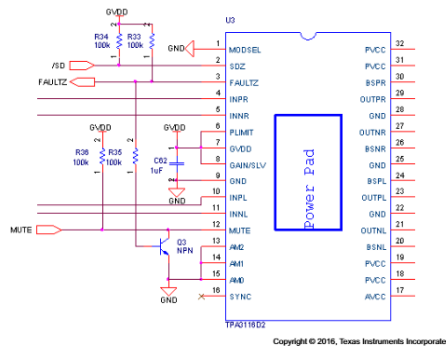
Figure 30. MUTE Driven by Inverted FAULTZ
