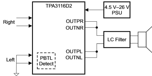
Figure 36. Mono Mode
