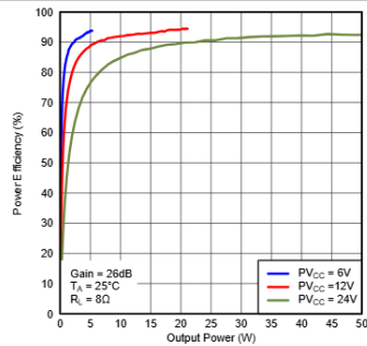
Figure 15. Power Efficiency (BTL) vs Output Power
