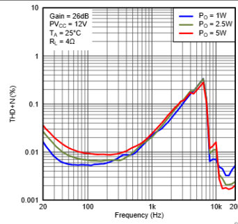
Figure 2. Total Harmonic Distortion + Noise (BTL) vs Frequency
