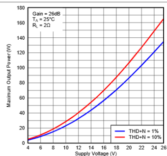
Figure 22. Maximum Output Power (PBTL) vs Supply Voltage
