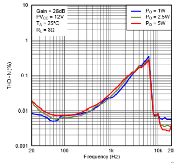
Figure 4. Total Harmonic Distortion + Noise (BTL) vs Frequency
