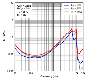
Figure 5. Total Harmonic Distortion + Noise (BTL) vs Frequency
