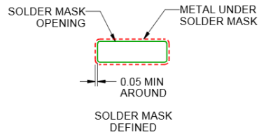
SOLDER MASK DETAILS NOT TO SCALE
