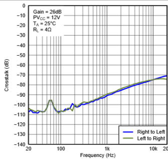
Figure 18. Crosstalk vs Frequency
