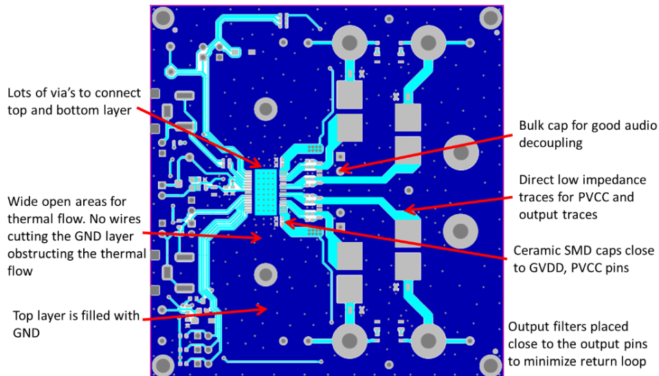
Figure 40. Layout Example Top
