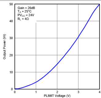
Figure 11. Output Power (BTL) vs Plimit Voltage
