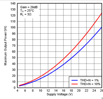
Figure 26. Maximum Output Power (PBTl) vs Supply Voltage
