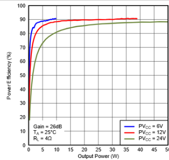
Figure 16. Power Efficiency (BTL) vs Output Power
