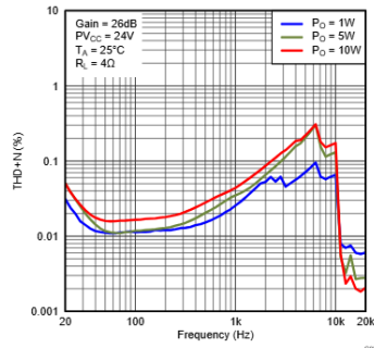
Figure 3. Total Harmonic Distortion + Noise (BTL) vs Frequency
