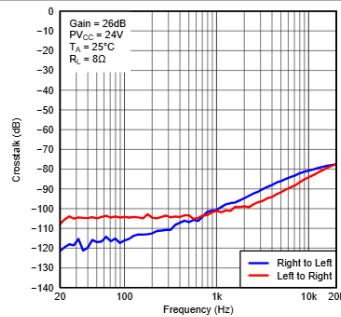
Figure 17. Crosstalk vs Frequency
