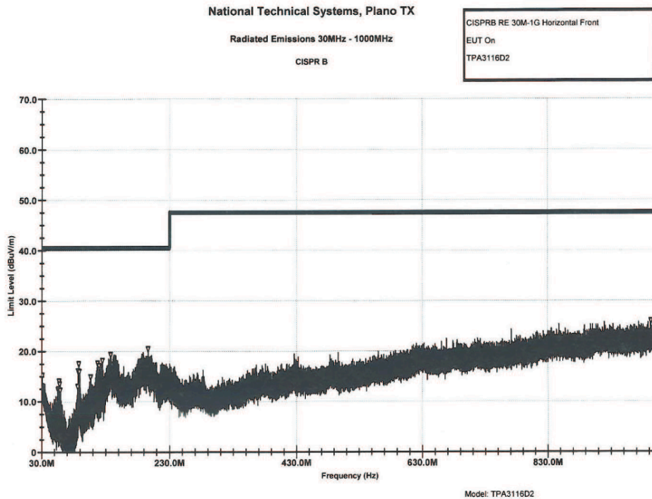
Figure 34. TPA311x2 Radiated Emissions
