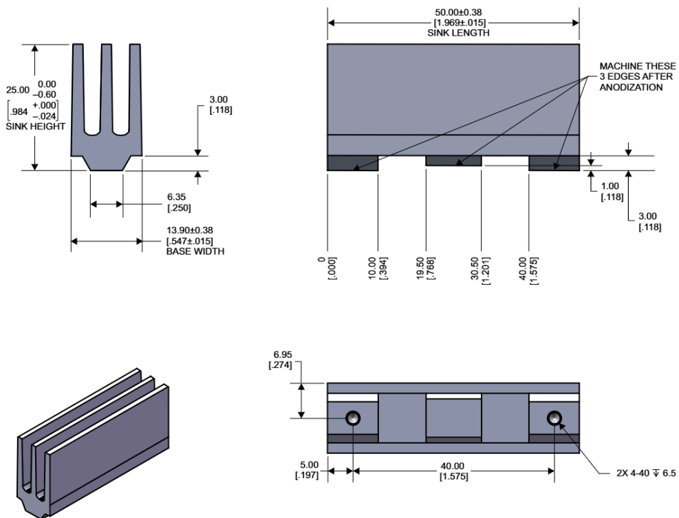
Figure 42. EVM Heatsink
