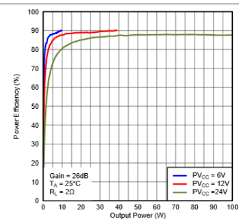
Figure 23. Power Efficiency (PBTL) vs Output Power
