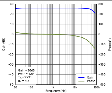
Figure 12. Gain/Phase (BTL) vs Frequency
