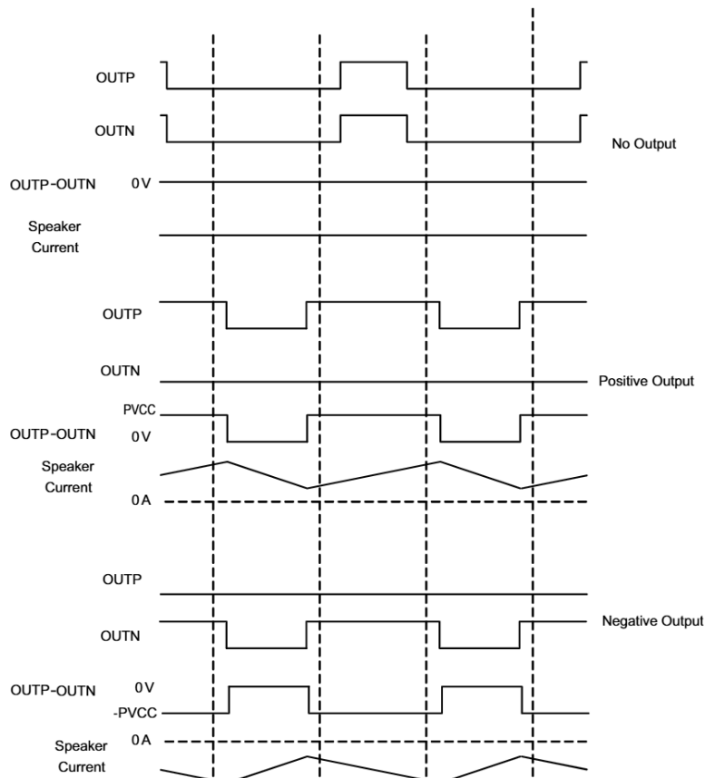
Figure 33. 1SPW Mode Modulation
