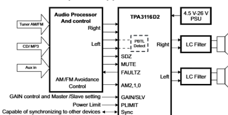
Simplified Application Circuit
