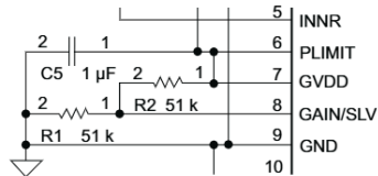
Figure 27. Gain, Master/Slave
