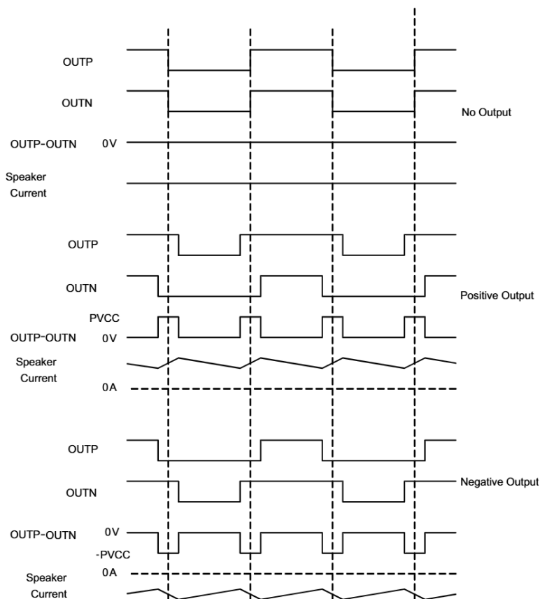
Figure 32. BD Mode Modulation
