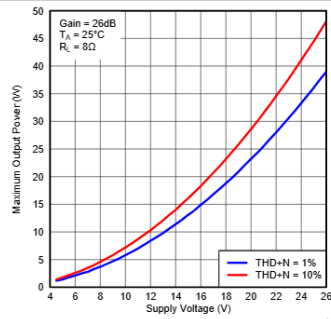
Figure 13. Maximum Output Power (BTL) vs Supply Voltage
