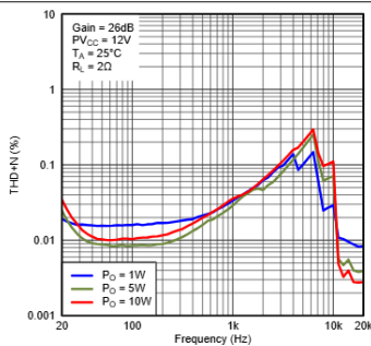
Figure 20. Total Harmonic Distortion + Noise (PBTL) vs Frequency
