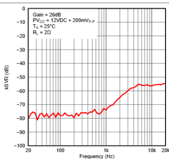
Figure 24. Supply Ripple Rejection Ratio (PBTL) vs Frequency
