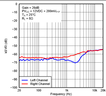
Figure 19. Supply Ripple Rejection Ratio (BTL) vs Frequency
