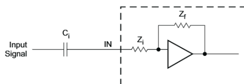
Figure 28. Input Impedance
