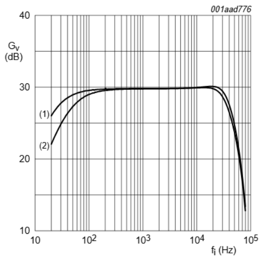
V_i = 100 \text{ mV (RMS)} ; R_i = 0 \Omega ; C_{se} = 1000 \mu\text{F} (1) V_P = 30 \text{ V} ; R_L = 2 \cdot 8 \Omega (2) V_P = 22 \text{ V} ; R_L = 2 \cdot 4 \Omega
