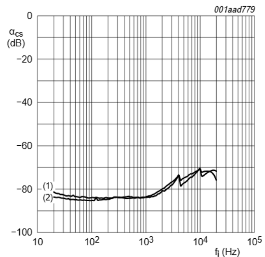
P_o = 1 \text{ W} ; Chv_{\text{pref}} = 47 \mu\text{F} (1) V_P = 22 \text{ V} ; R_L = 2 \cdot 4 \Omega (2) V_P = 30 \text{ V} ; R_L = 2 \cdot 8 \Omega
