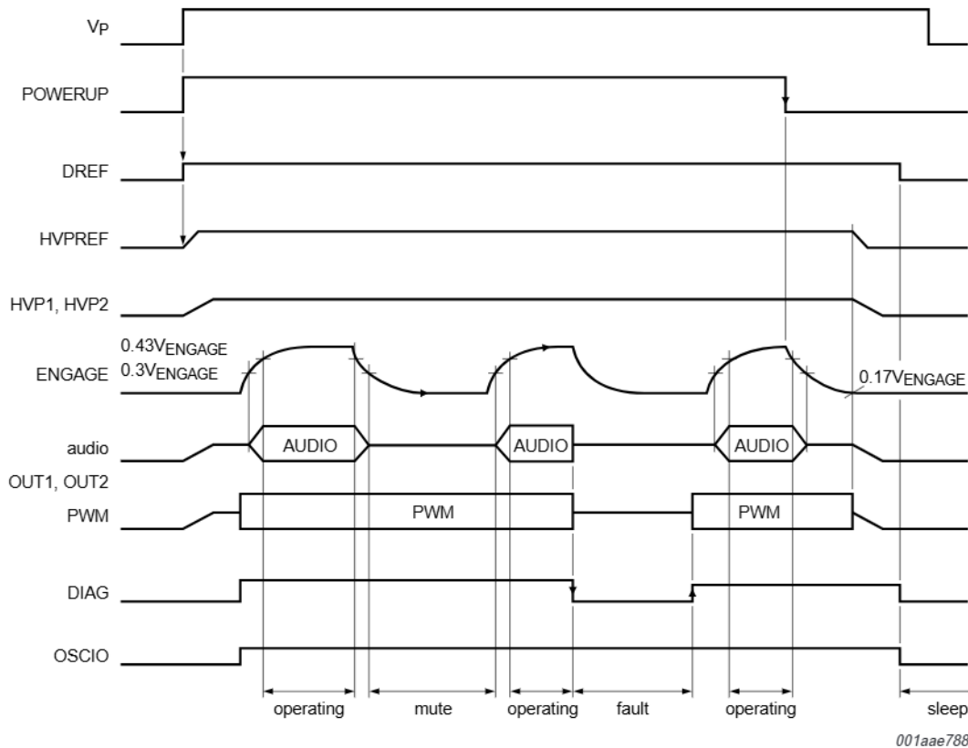
Fig 3. Start-up sequence
