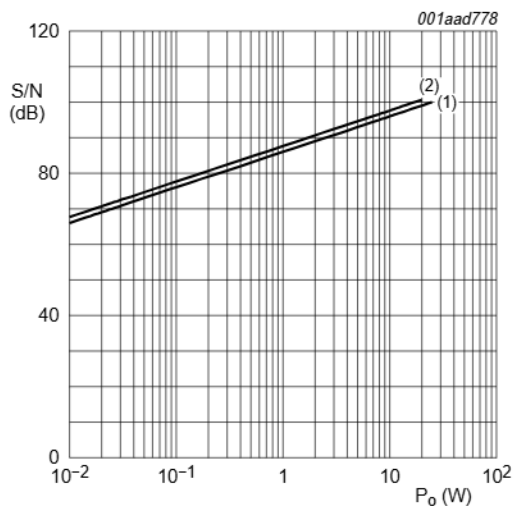
V_P = 22 \text{ V} ; R_i = 0 \Omega ; 20 kHz brick-wall filter AES17 (1) R_L = 2 \cdot 4 \Omega (2) R_L = 2 \cdot 8 \Omega
