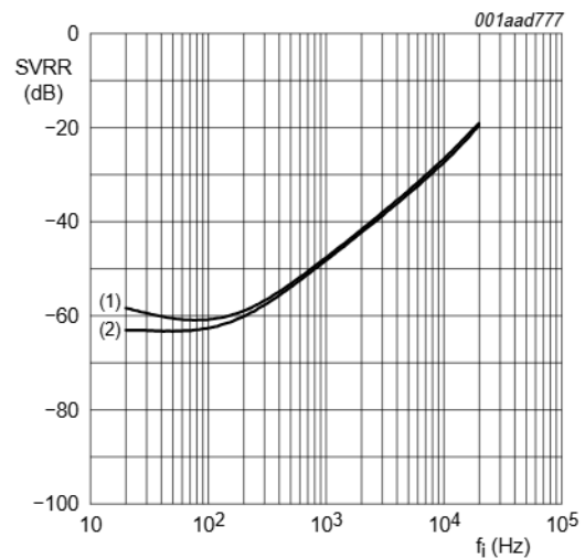
V_{\text{ripple}} = 500 \text{ mV (RMS)} referenced to ground; R_i = 0 \Omega (shorted input) (1) V_P = 30 \text{ V} ; R_L = 2 \cdot 8 \Omega (2) V_P = 22 \text{ V} ; R_L = 2 \cdot 4 \Omega
