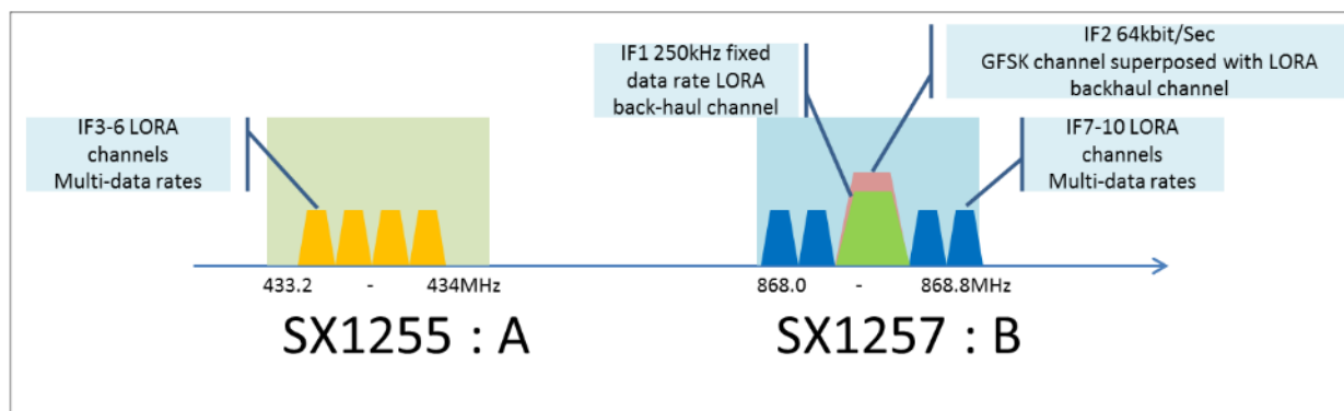
Figure 11: Radio Spectrum
