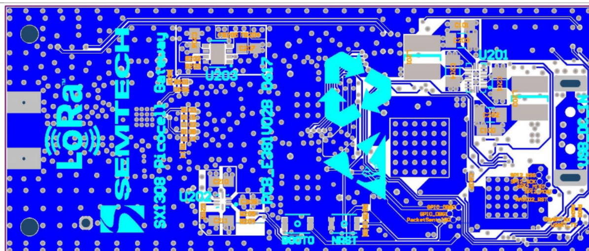
Figure 17: PCB Layout Example
