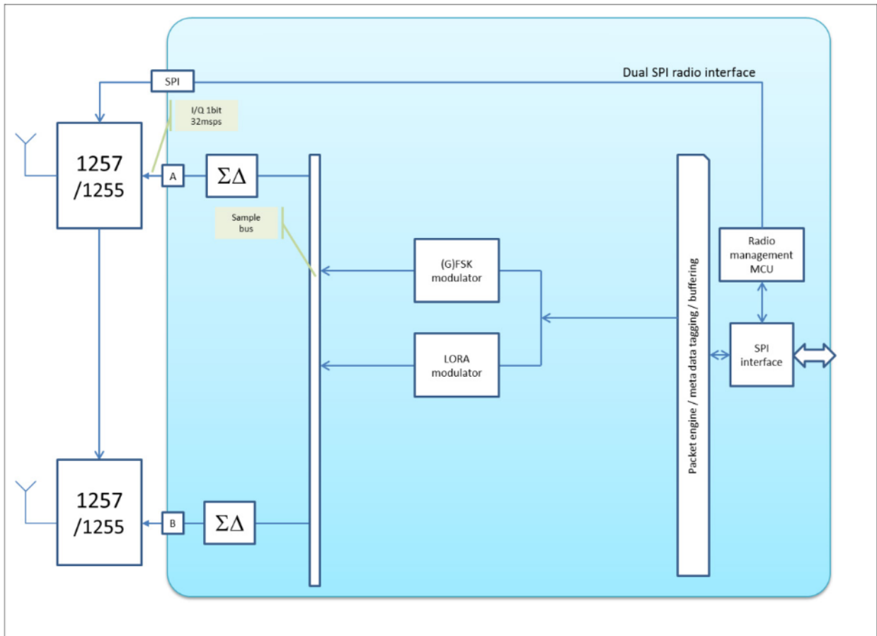
Figure 15: Transmission Schematics
