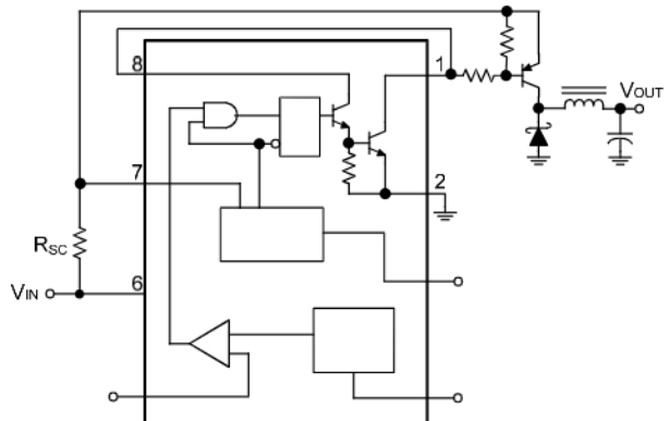
2b. External PNP Saturated Switch
