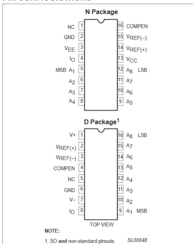
Figure 1. Pin Configurations
