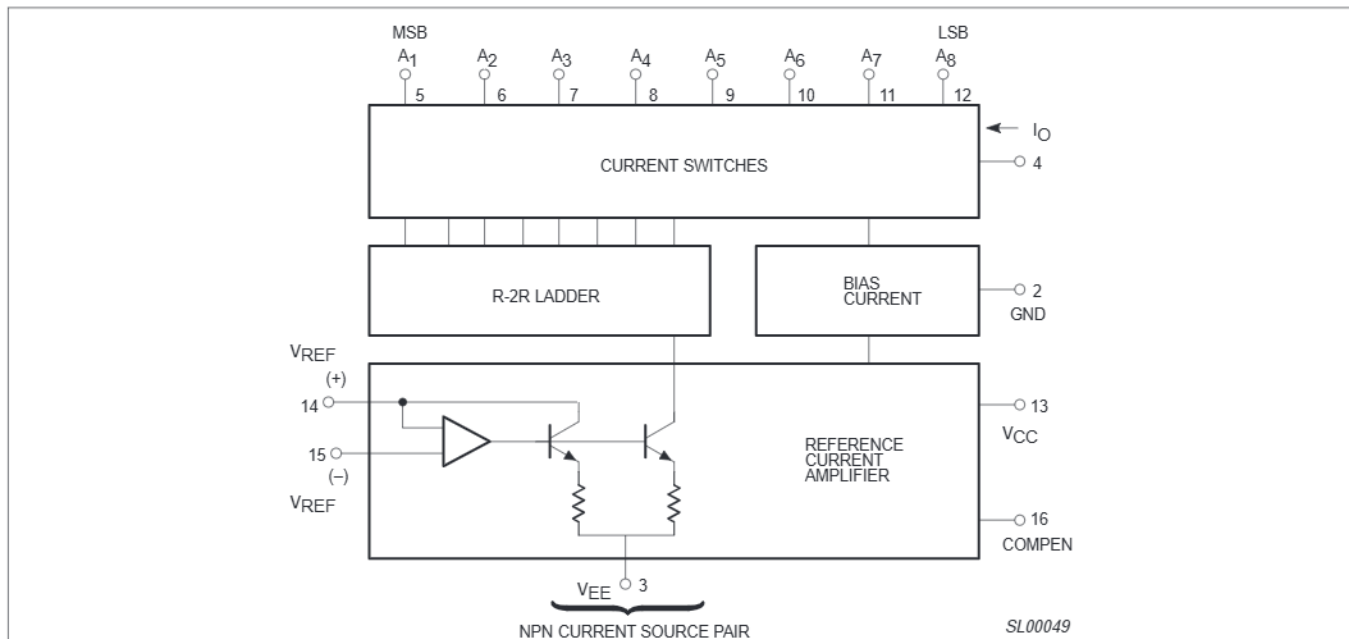
Figure 2. Block Diagram
