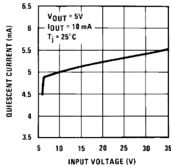
Figure 12. Quiescent Current
