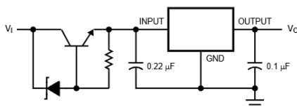
Figure 23. High Input Voltage Circuit implementation With Transistor
