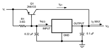
Figure 24. High Current Voltage Regulator
