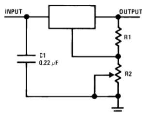
Figure 21. Adjustable Output Regulator
