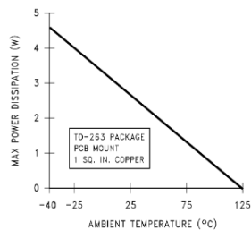
Figure 30. Maximum Power Dissipation vs T_{\text{AMB}} for the DDPAK/TO-263 Package
