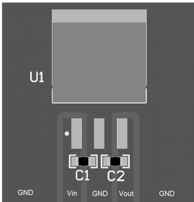
Figure 27. Layout Example DDPAK
