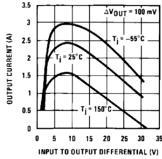
Figure 8. Dropout Characteristics
