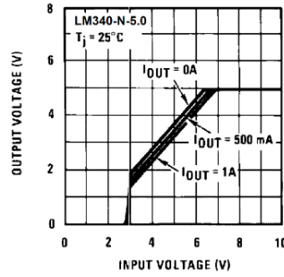
Figure 8. Dropout Characteristics
