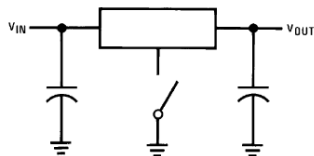
Figure 16. Regulator Floating Ground
