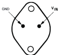
LM340K-5.0 NDS Package 2-Pin TO-3 Top View
