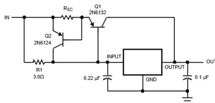
Figure 25. High Output Current With Short-Circuit Protection
