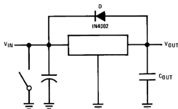
Figure 15. Input Short
