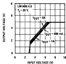
Figure 19. V_{OUT} vs V_{IN} , V_{OUT} = 5 V
