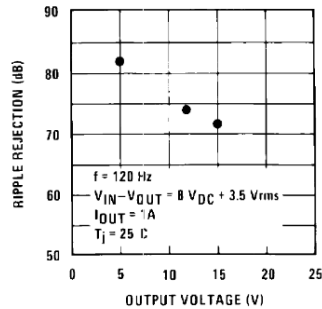
Figure 6. Ripple Rejection
