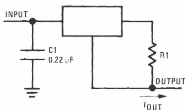
Figure 20. Current Regulator
