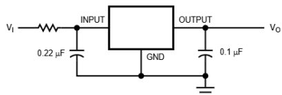
Figure 22. High Input Voltage Circuit With Series Resistor
