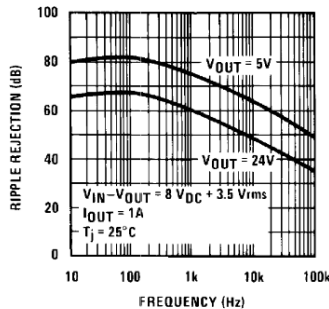
Figure 5. Ripple Rejection
