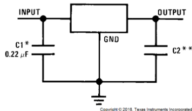
Figure 18. Fixed Output Voltage Regulator
