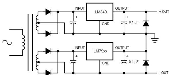
Figure 26. LM340 Used With Negative Regulator LM79xx
