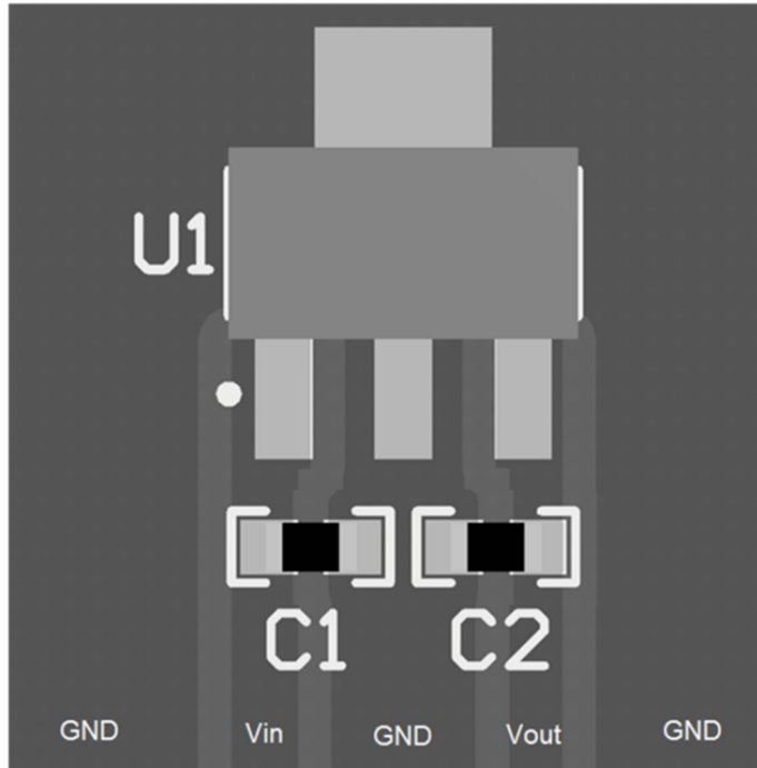
Figure 28. Layout Example SOT-223
