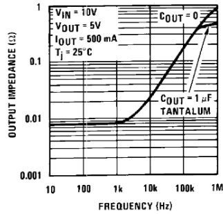
Figure 7. Output Impedance
