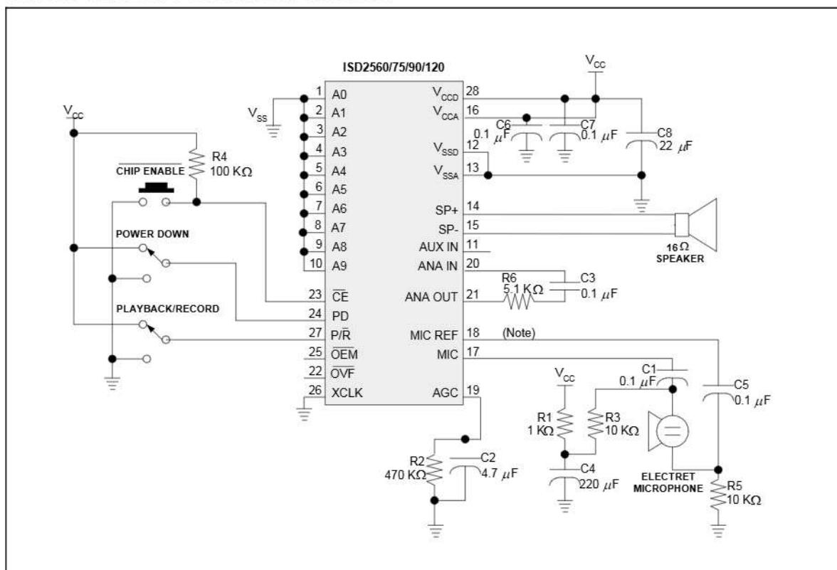
FIGURE 5: DESIGN SCHEMATIC
