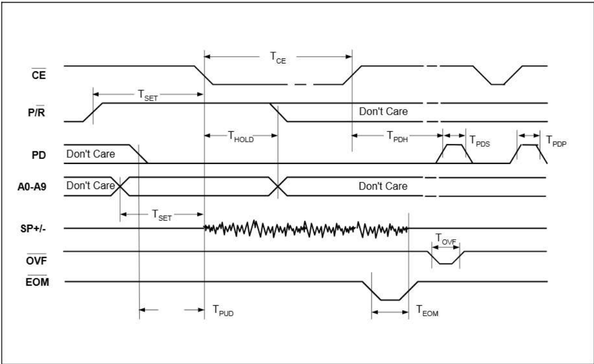
FIGURE 2: PLAYBACK
