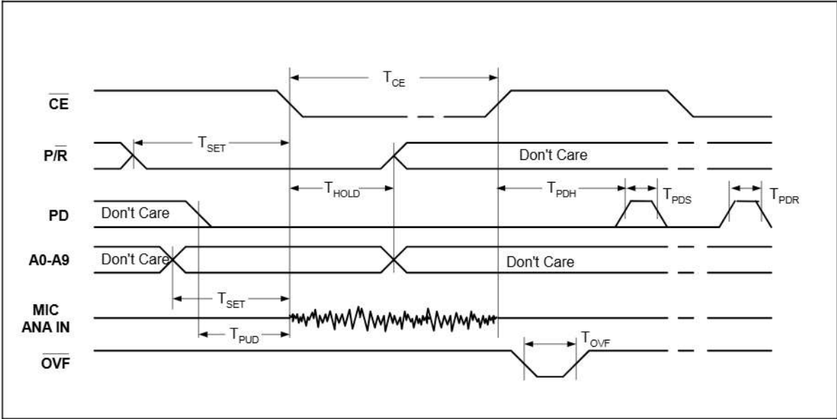
FIGURE 1: RECORD
