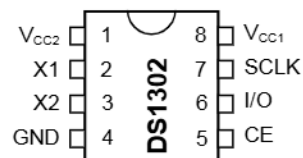
DIP (300 mils)
