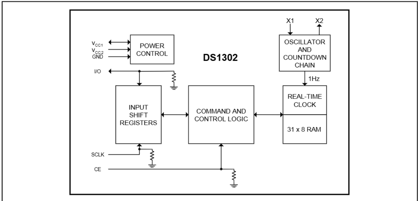
Figure 1. Block Diagram
