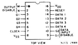
TERMINAL ASSIGNMENT
