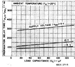
Fig. 6 - Typical propagation delay time vs. load capacitance (clock to Q).
