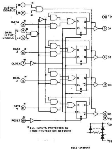
Fig. 8 - CD4076B logic diagram.
