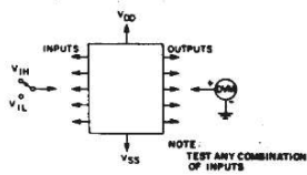
Fig. 12 — Input voltage test circuit.
