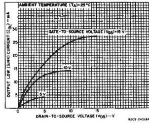
Fig.1 — Typical output low (sink) current characteristics.
