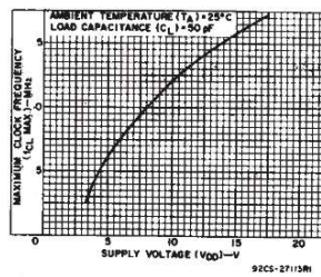
Fig.9 — Typical maximum clock input frequency vs. supply voltage.
