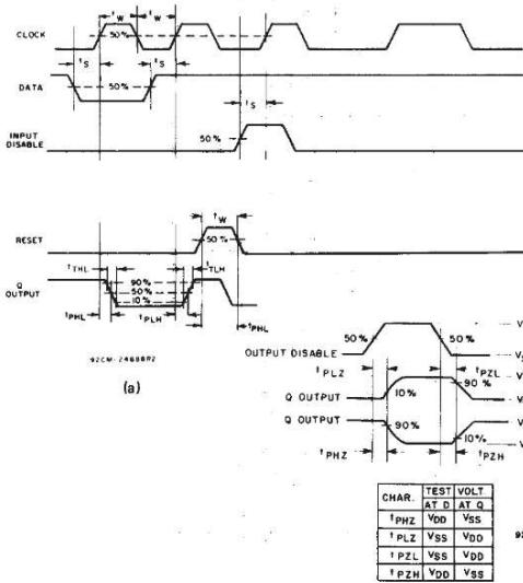
Fig. 5 - Functional waveforms for CD4076B.
