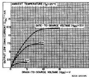
Fig.2 — Minimum output low (sink) current characteristics.
