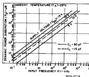
Fig.10 — Typical dynamic power dissipation vs. frequency.
