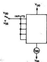
Fig. 11 — Quiescent device current test circuit.
