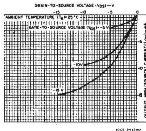
Fig. 4 - Minimum output high (source) current characteristics.
