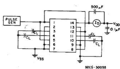
Fig. 13 - Dynamic power dissipation test circuit.
