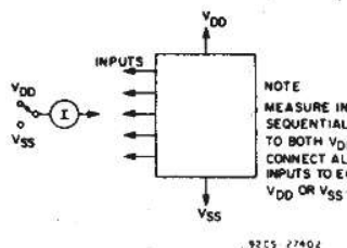
Fig. 12 - Input-current test circuit.
