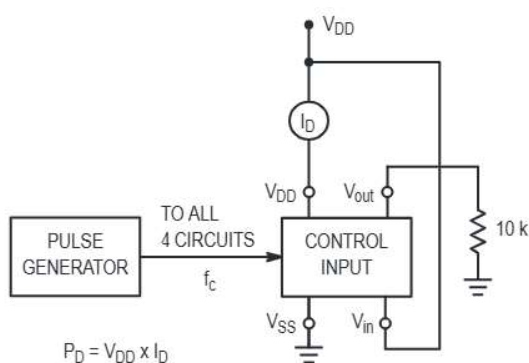
Figure 2. Quiescent Power Dissipation Test Circuit
