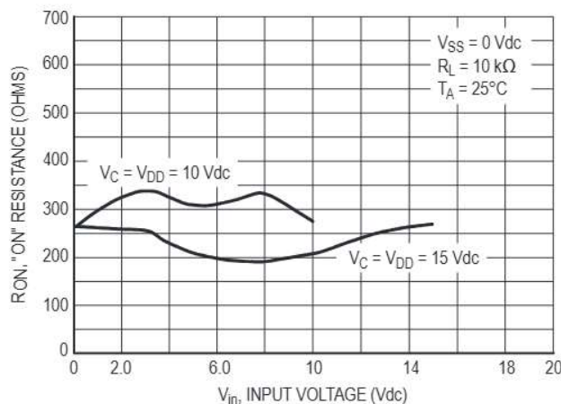
Figure 5. V_{SS} = 0 V
