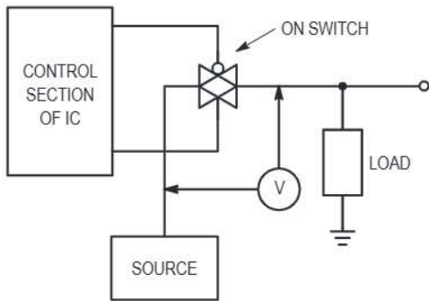
Figure 14. ΔV Across Switch
