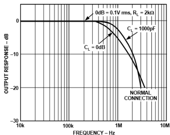
Figure 15. Frequency Response
