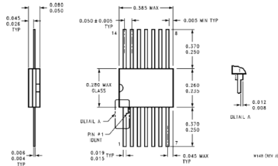
14-Lead Ceramic Flat Package (W) Order Number 54121FMBQ or DM54121W NS Package Number W14B
