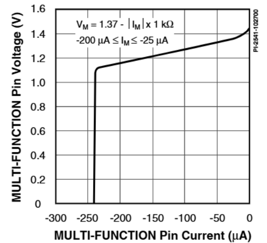
Figure 64b. MULTI-FUNCTION Pin Voltage vs. Current (Expanded).
