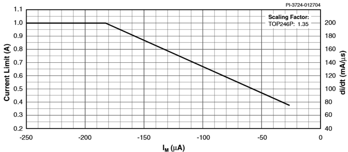
Figure 56a. Current Limit vs. MULTI-FUNCTION Pin Current (TOP246P only).
