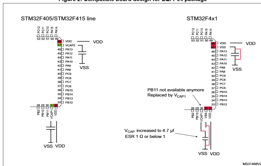
Figure 2. Compatible board design for LQFP64 package
