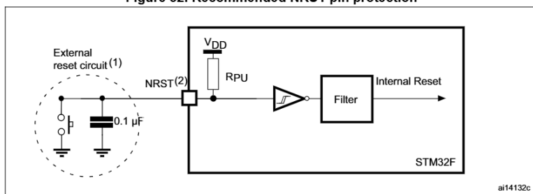
Figure 32. Recommended NRST pin protection
