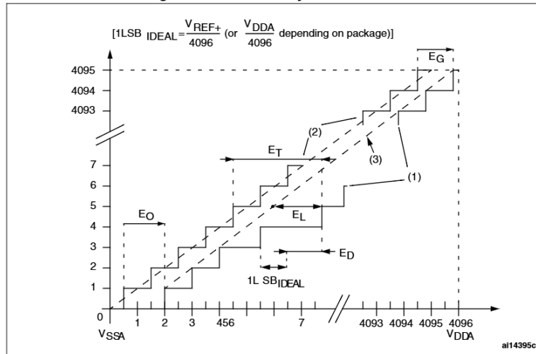
Figure 40. ADC accuracy characteristics
