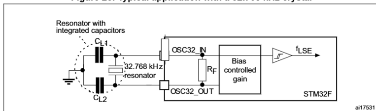
Figure 25. Typical application with a 32.768 kHz crystal
