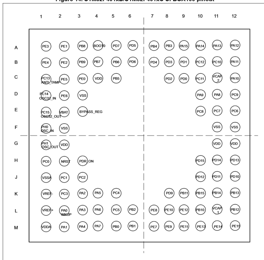
Figure 14. STM32F401xB/STM32F401xC UFBGA100 pinout
