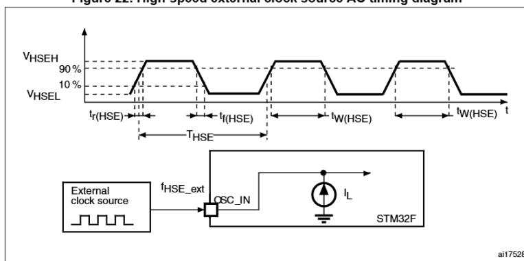
Figure 22. High-speed external clock source AC timing diagram
