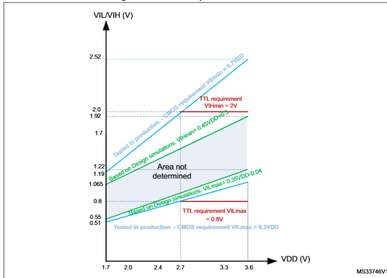
Figure 30. FT I/O input characteristics
