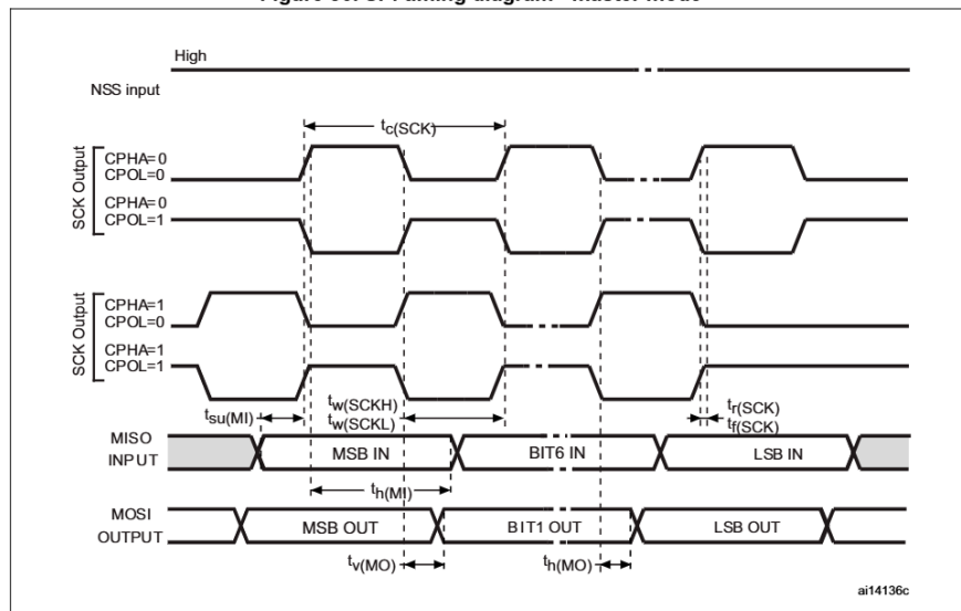
Figure 36. SPI timing diagram - master mode (1)
