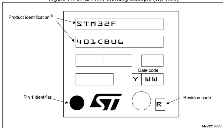
Figure 51. UFQFPN48 marking example (top view)
