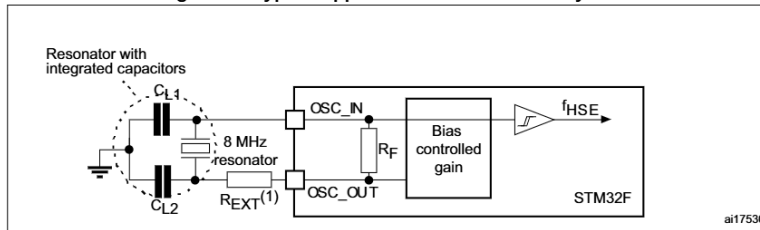
Figure 24. Typical application with an 8 MHz crystal
