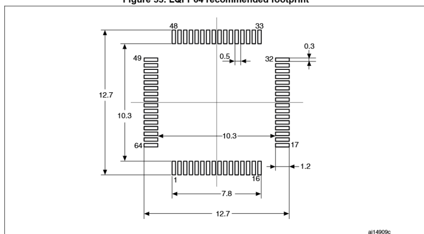
Figure 53. LQFP64 recommended footprint
