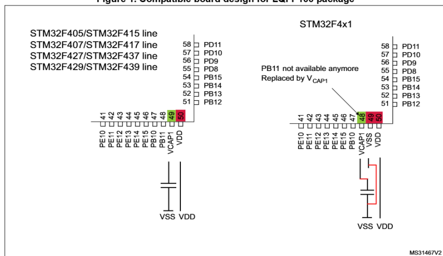
Figure 1. Compatible board design for LQFP100 package
