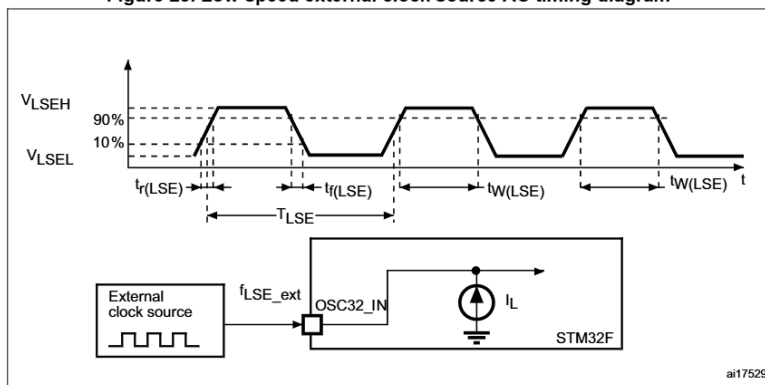
Figure 23. Low-speed external clock source AC timing diagram
