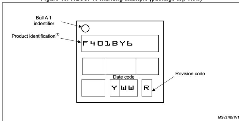
Figure 48. WLCSP49 marking example (package top view)
