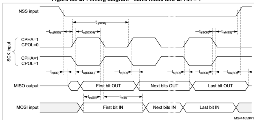
Figure 35. SPI timing diagram - slave mode and CPHA = 1 (1)
