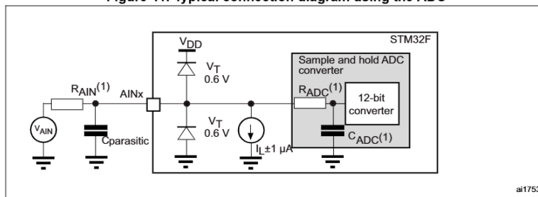
Figure 41. Typical connection diagram using the ADC
