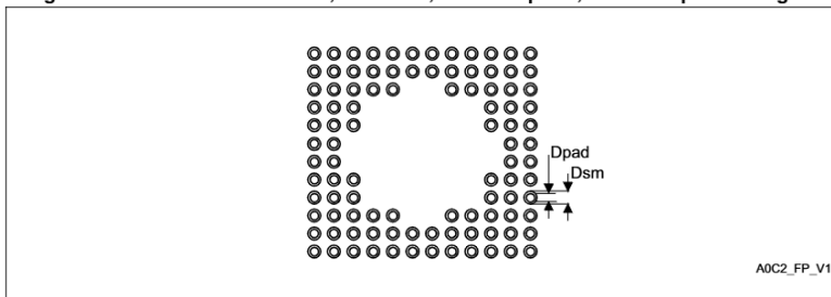
array package recommended footprint
