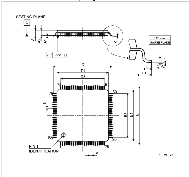
Figure 55. LQFP100 - 100-pin, 14 x 14 mm, 100-pin low-profile quad flat package outline
