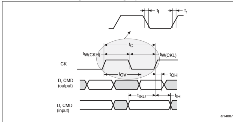
Figure 45. SD default mode
