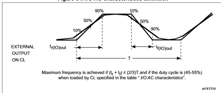
Figure 31. I/O AC characteristics definition
