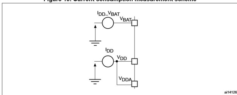
Figure 19. Current consumption measurement scheme
