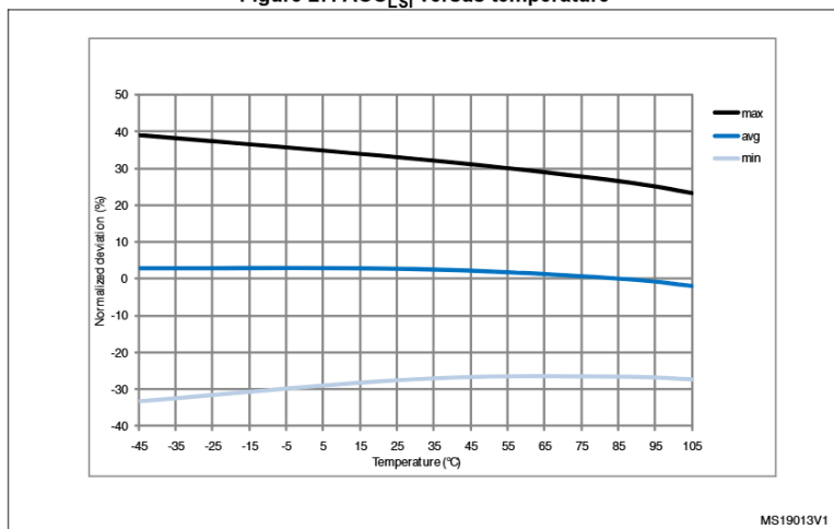
Figure 27. ACC_{LSI} versus temperature
