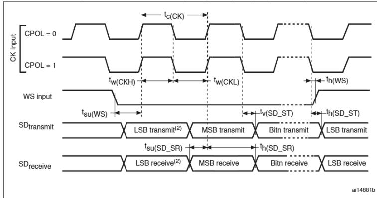
Figure 37. I 2 S slave timing diagram (Philips protocol) (1)
