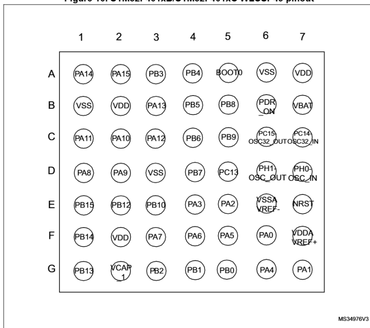
Figure 10. STM32F401xB/STM32F401xC WLCSP49 pinout
