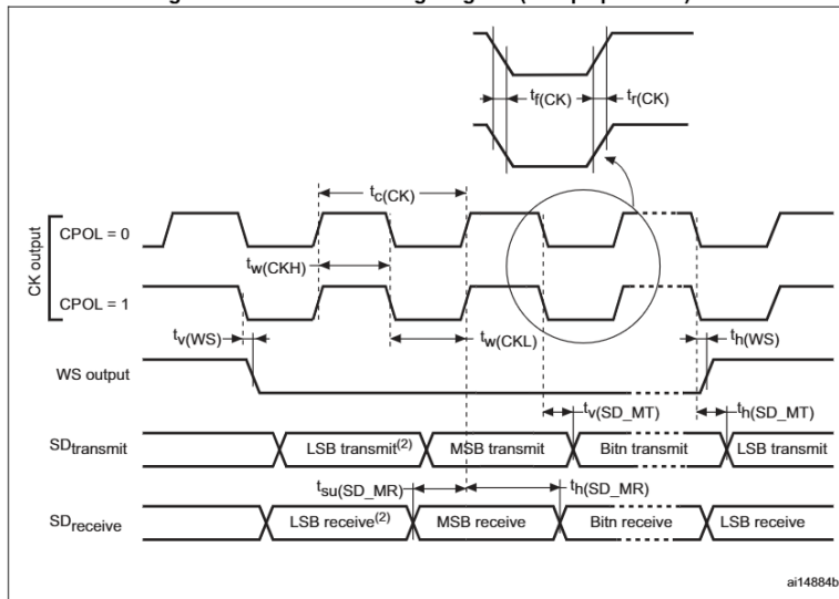
Figure 38. I 2 S master timing diagram (Philips protocol) (1)
