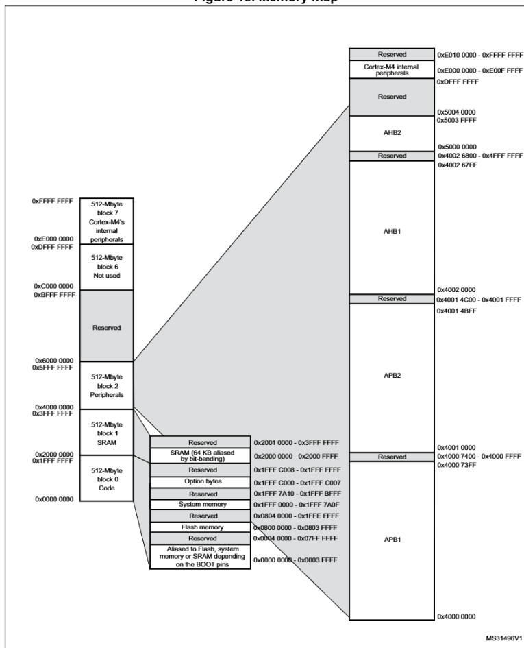
Figure 15. Memory map
