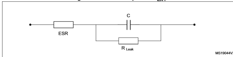
Figure 20. External capacitor C_{EXT}
