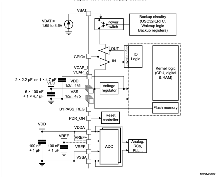
Figure 18. Power supply scheme
