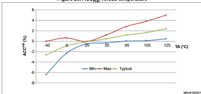
Figure 26. ACC_{HSL} versus temperature
