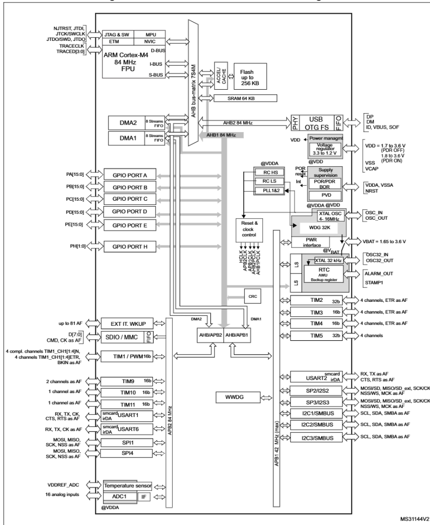
Figure 3. STM32F401xB/STM32F401xC block diagram
