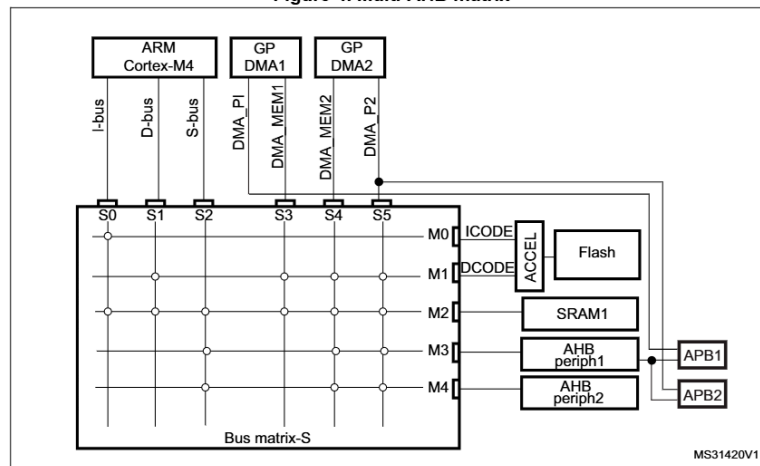
Figure 4. Multi-AHB matrix
