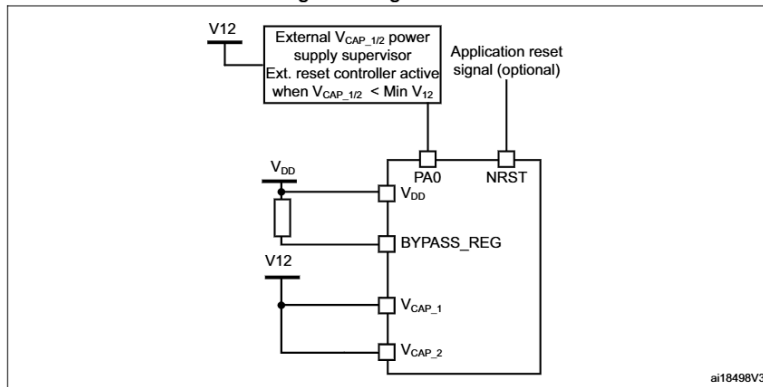
Figure 7. Regulator OFF
