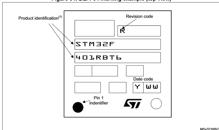
Figure 54. LQFP64 marking example (top view)
