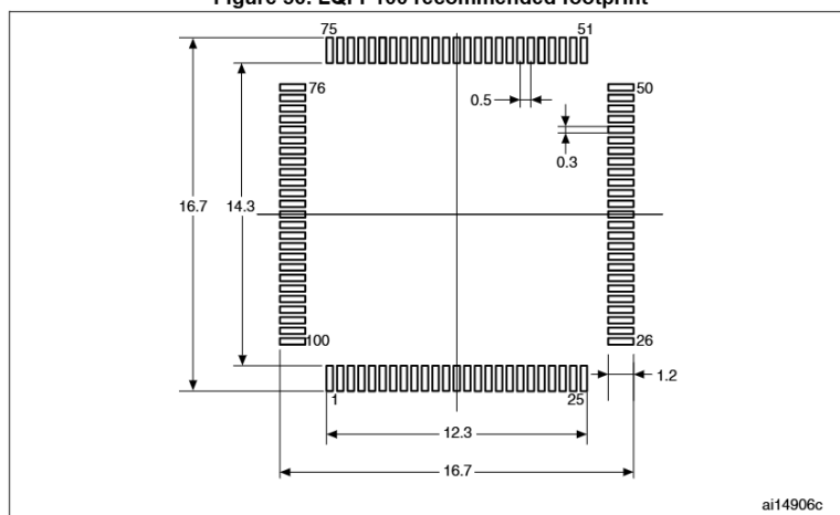
Figure 56. LQFP100 recommended footprint
