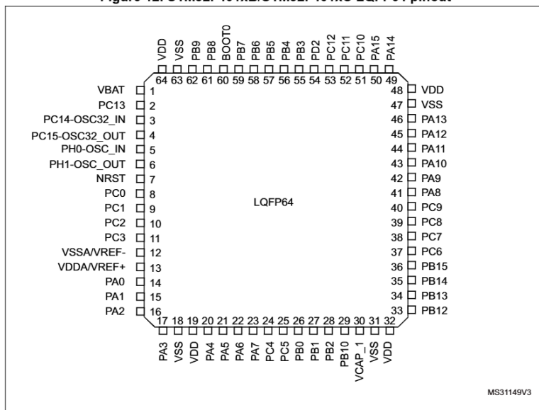
Figure 12. STM32F401xB/STM32F401xC LQFP64 pinout
