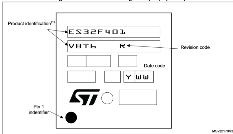
Figure 57. LQFP100 marking example (top view)
