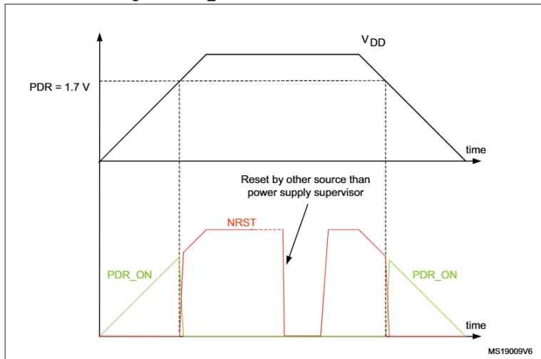
Figure 6. PDR_ON control with internal reset OFF
