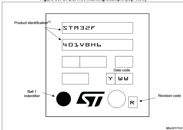
Figure 60. UFBGA100 marking example (top view)
