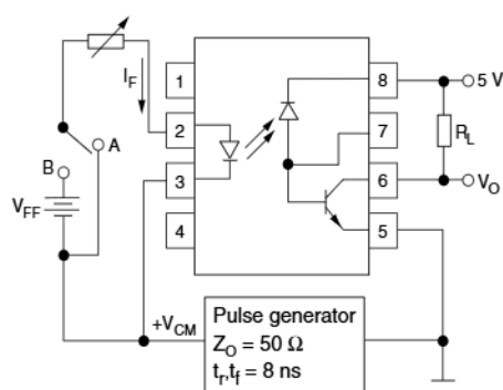
Fig. 2 Common-Mode Interference Immunity
