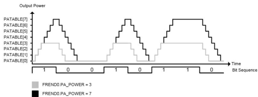
Figure 23: Shaping of ASK Signal
