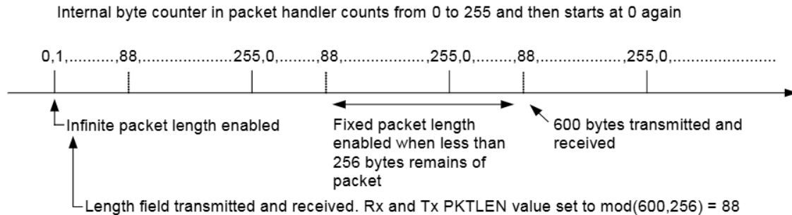
Figure 12: Packet Length > 255
