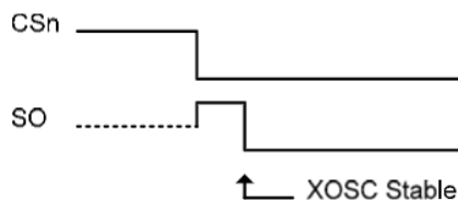
Figure 17: Power-On Reset
