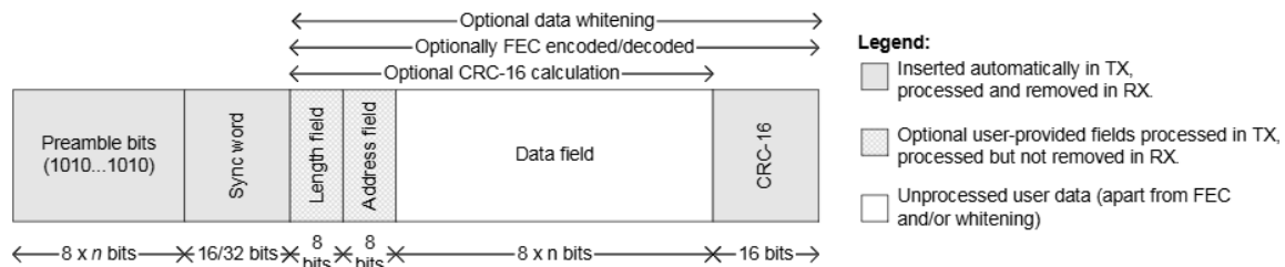
Figure 11: Packet Format
