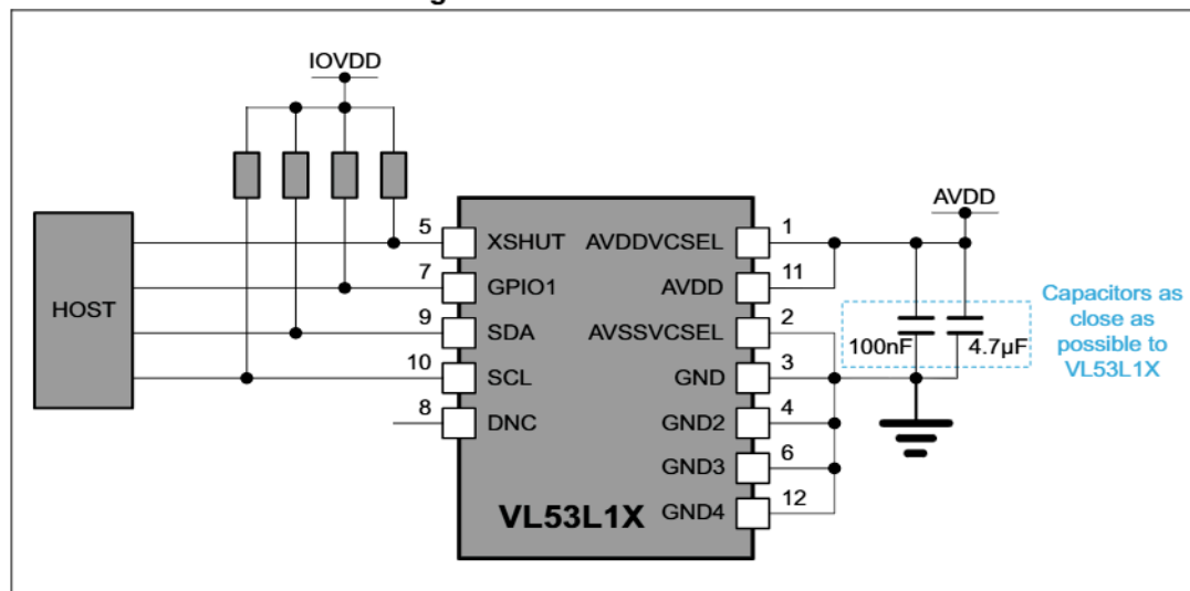
Figure 3. VL53L1X schematic
