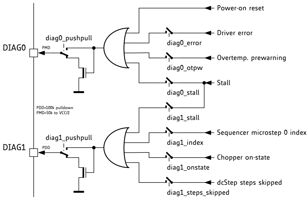
Figure 14.1 DIAG outputs
