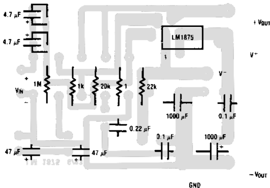
Figure 14. Split Supply
