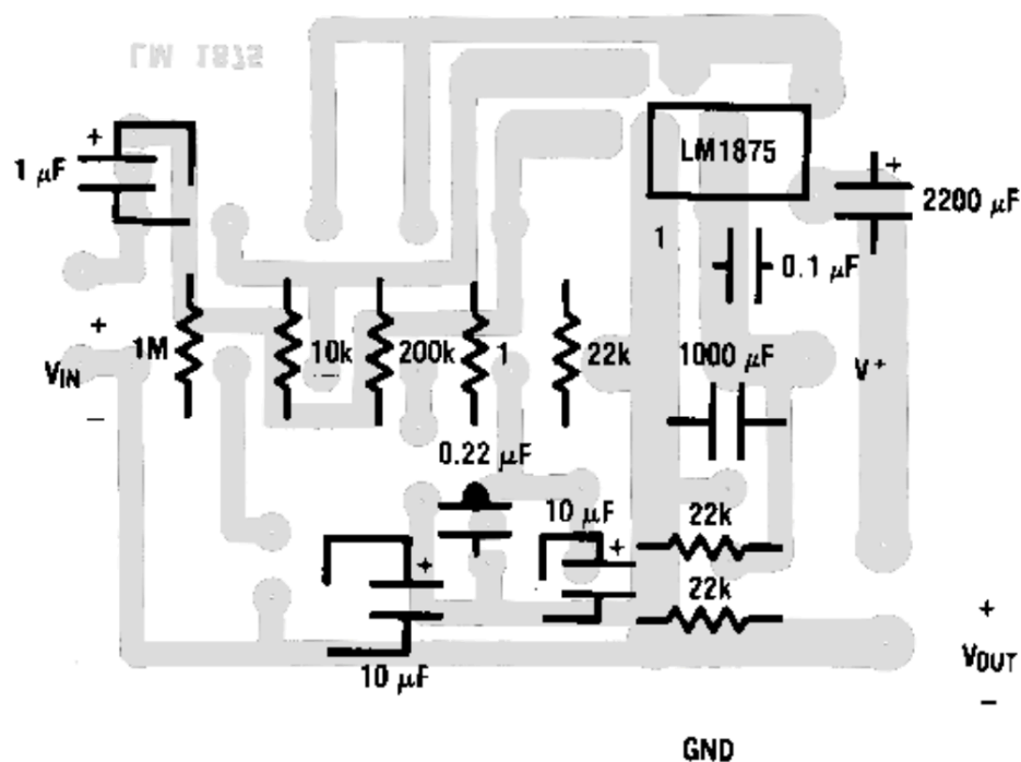
Figure 15. Single Supply
