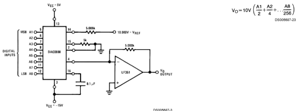
FIGURE 1. +10V Output Digital to Analog Converter (Note 8)
