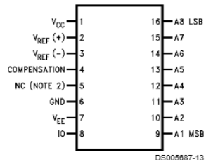
Small-Outline Package
