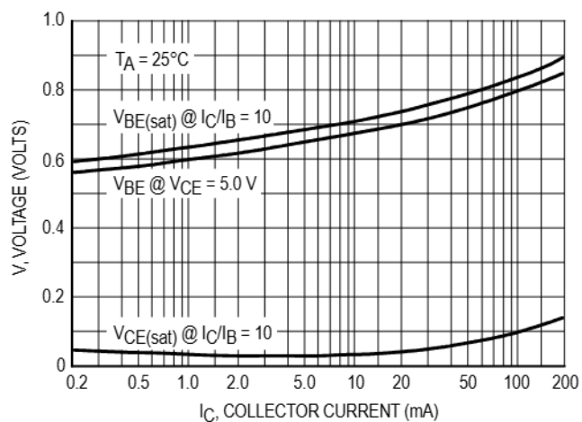
Figure 8. "On" Voltage
