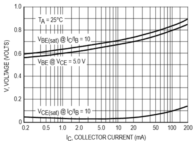
Figure 8. "On" Voltage
