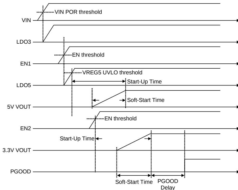
Figure 5. RT8249A/C Timing
