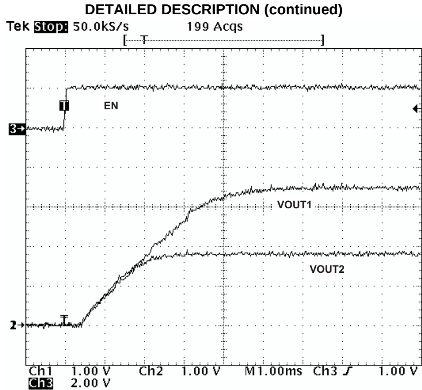
Figure 37. Simultaneous Startup With Tracking Resistor
