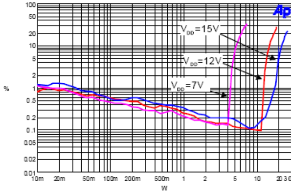
7. THD+N vs. Power
