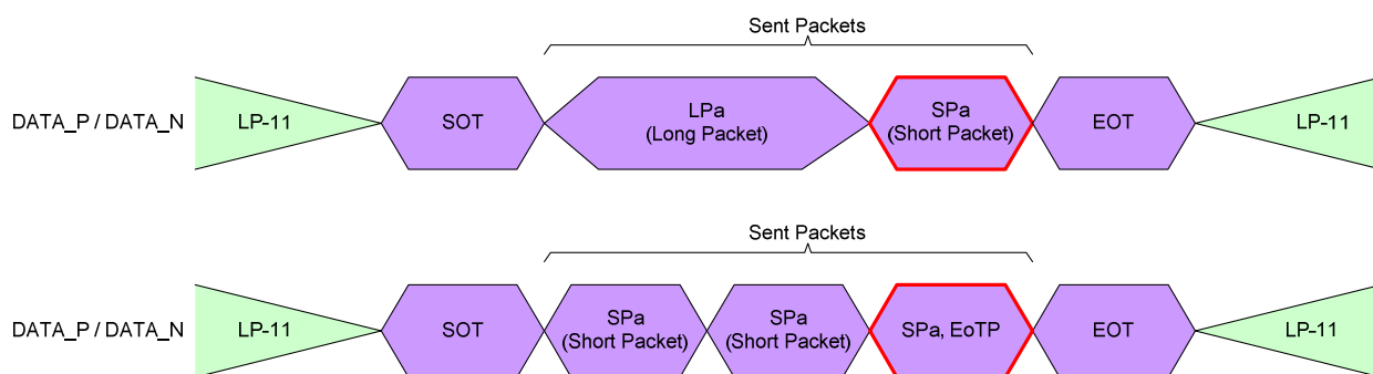
Figure 75: End of Transmission Packet (EoTP) – Examples
