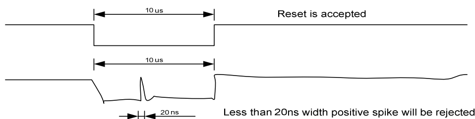
Figure 137: Positive Noise Pulse during Reset Low
