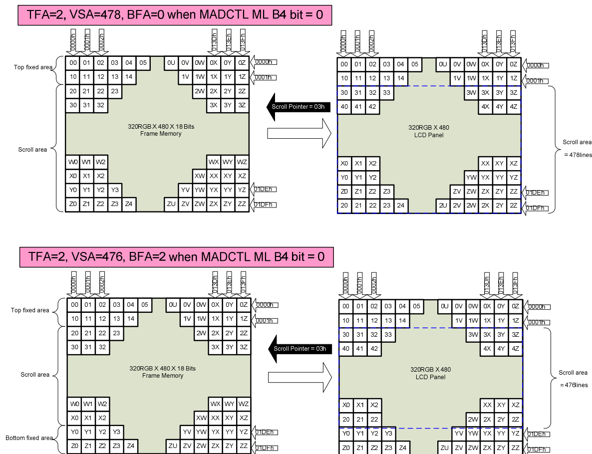
Figure 128: Vertical Scrolling Mode Function
