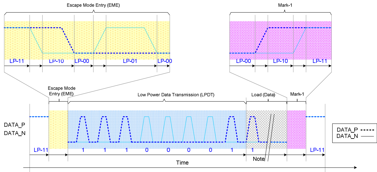
Figure 31: Low-Power Data Transmission (LPDT)
