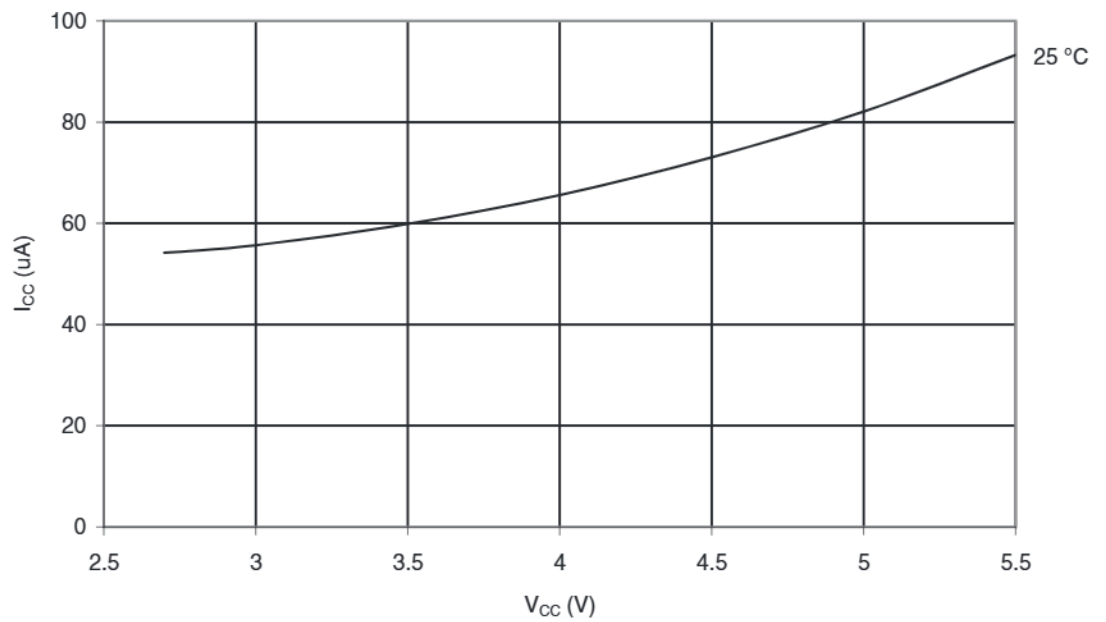
Figure 26-23. Standby Supply Current vs. V_{CC} (6 MHz Resonator, Watchdog Timer Disabled)
