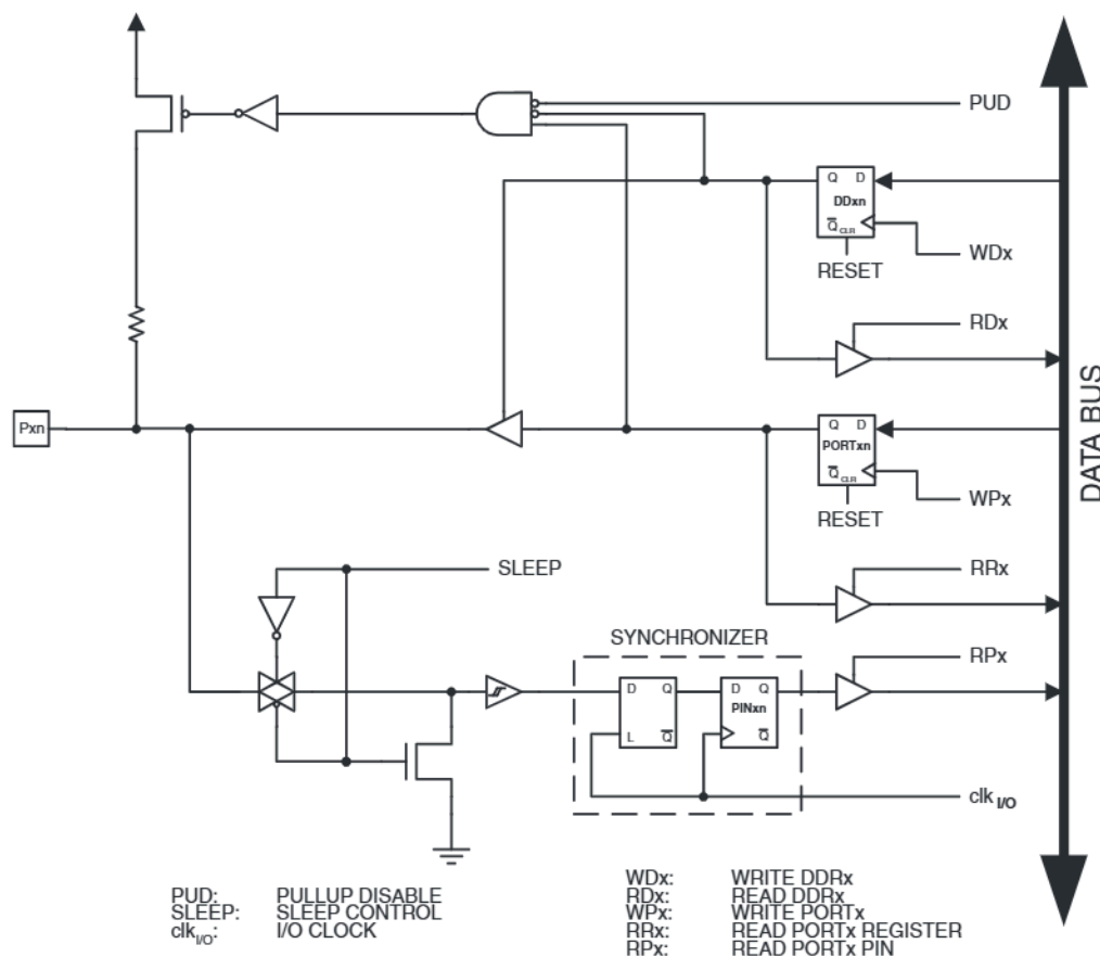
Figure 12-2. General Digital I/O (1)
