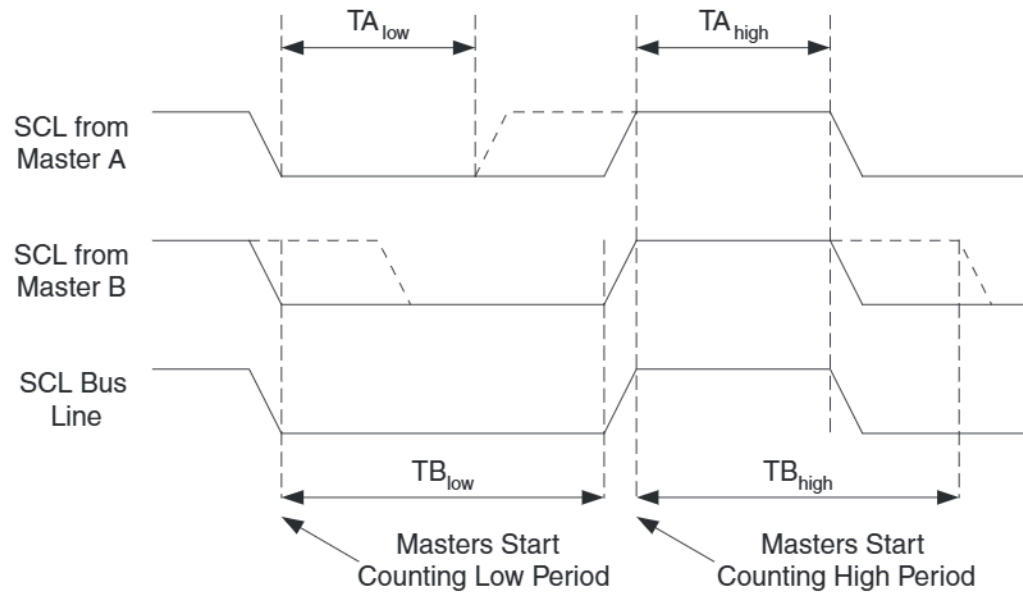
Figure 20-8. SCL Synchronization Between Multiple Masters
