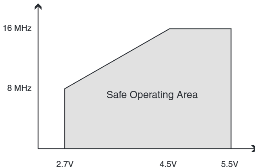
Figure 25-1. Maximum Frequency vs. V CC
