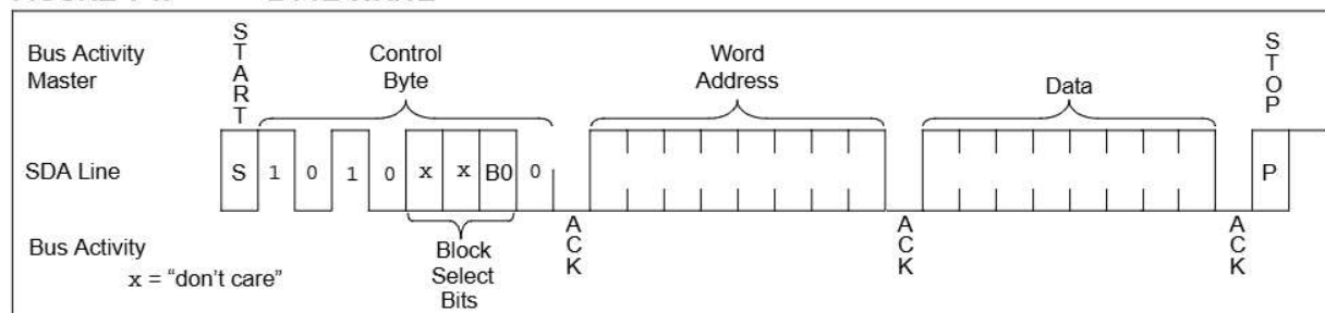
FIGURE 4-1: BYTE WRITE
