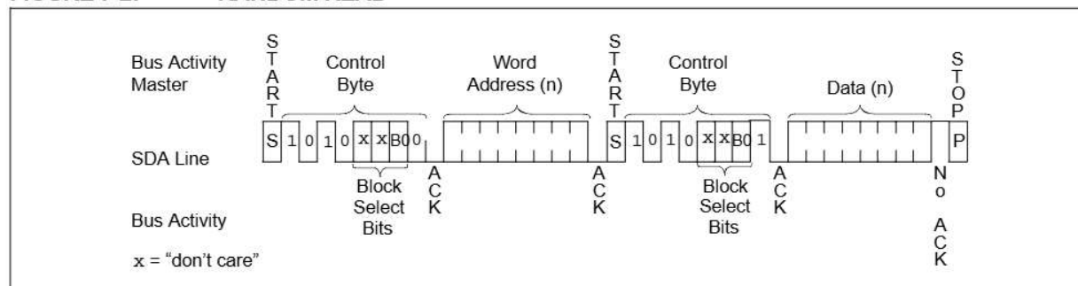
FIGURE 7-2: RANDOM READ
