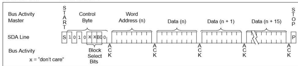
FIGURE 4-2: PAGE WRITE
