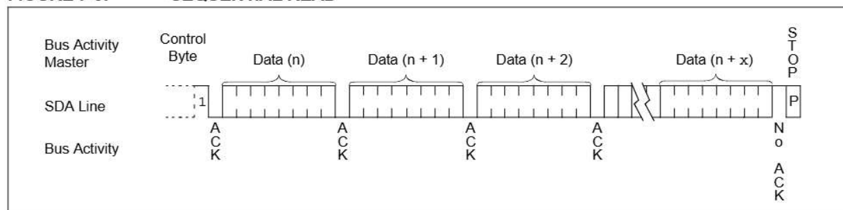
FIGURE 7-3: SEQUENTIAL READ
