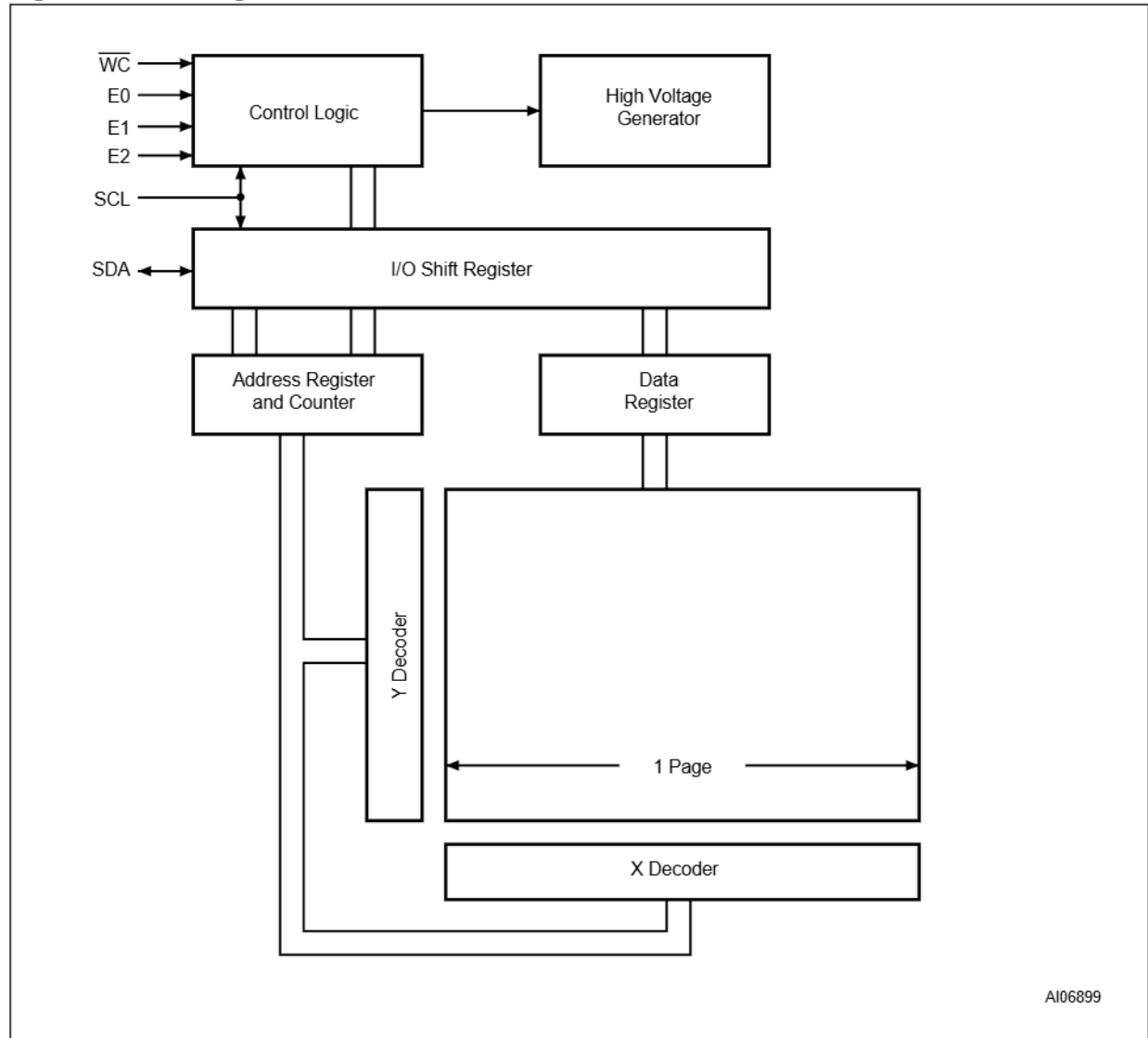
Figure 6. Block Diagram
