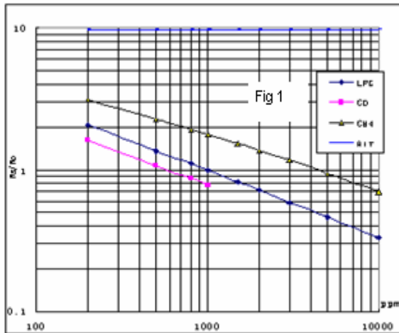
Fig.1 shows the typical sensitivity characteristics of the MQ-9, ordinate means resistance ratio of the sensor ( R_s/R_0 ), abscissa is concentration of gases. R_s means resistance in different gases, R_0 means resistance of sensor in 1000ppm LPG. All test are under standard test conditions.
