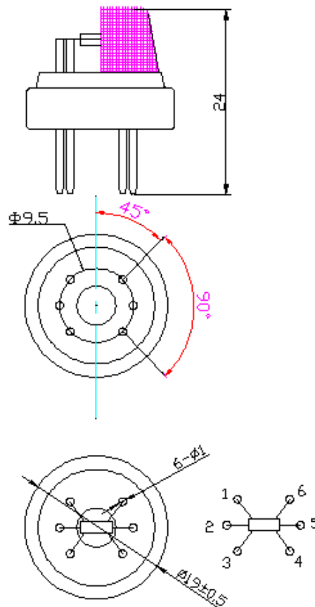
Fig1.Sensor Structure
