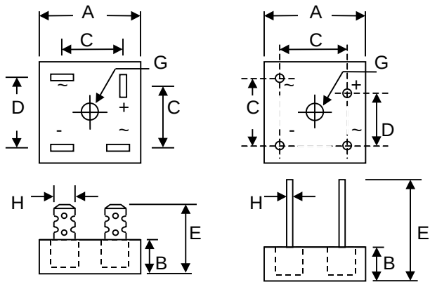
KBPC
